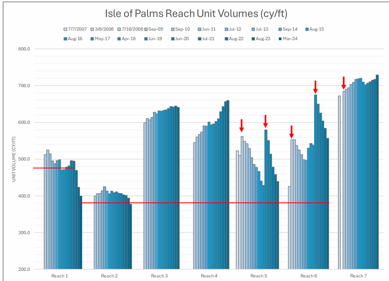
FIGURE 8. Reach Unit Volumes at Isle of Palms. Minimum healthy beach volumes are shown in the red line.
